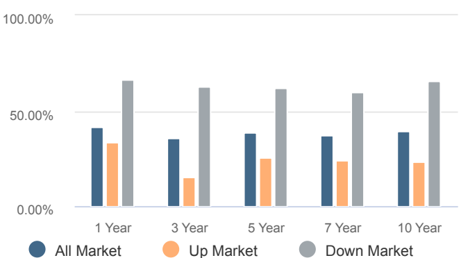
Returns Consistency
